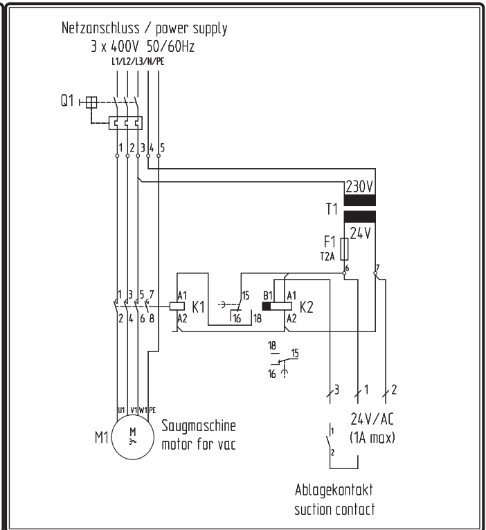
Schaltplan EXCOM hybrid 2/5 - 400V
