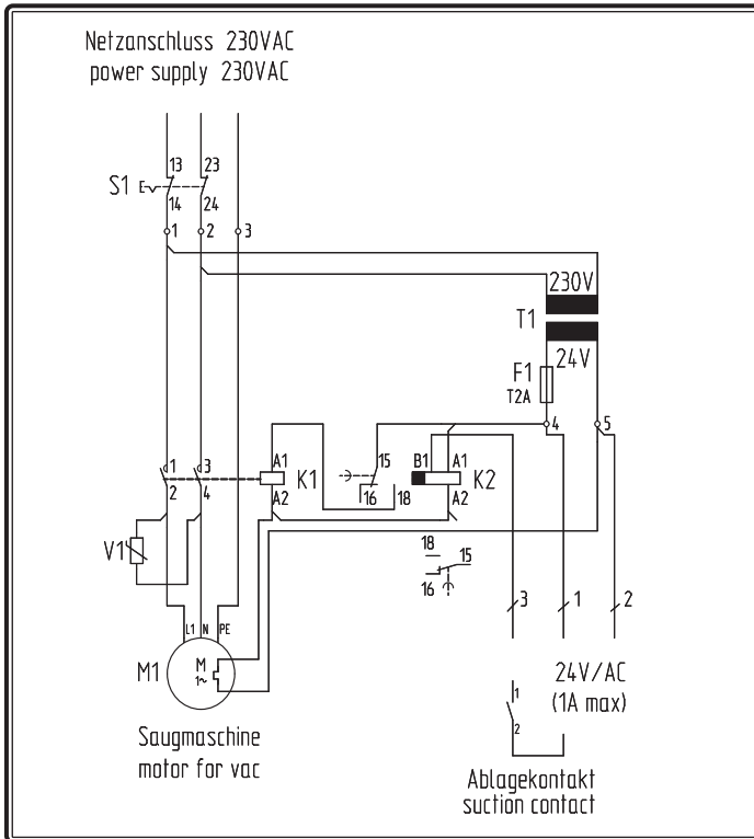
Schaltplan EXCOM hybrid 2/5 - 230V
